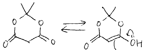
Meldrum's acid
