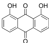
1,8-dihydroxyanthraquinone (1,8-HOAQ, chrysazine)
